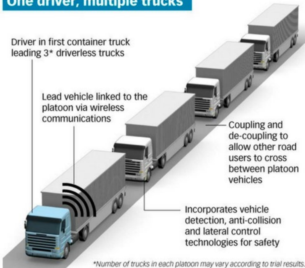
Figure 7 – Truck platooning 41
